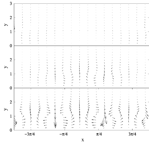
FIGURE 4 Time series of flow pattern during hole formation. ( Top panel ) At \bar{t} = 0 , random initial conditions produce a small flow. ( Middle panel ) At \bar{t} = 4 , the bacteria have started to aggregate in three locations. At these locations there is a strong downward flow. In locations where there are fewer bacteria, the return flow dominates the flow produced by the bacteria, setting up circular flow patterns. ( Bottom panel ) Flow at \bar{t} = 8 . Scaling of arrows in top panel is larger to make the arrows more visible.
